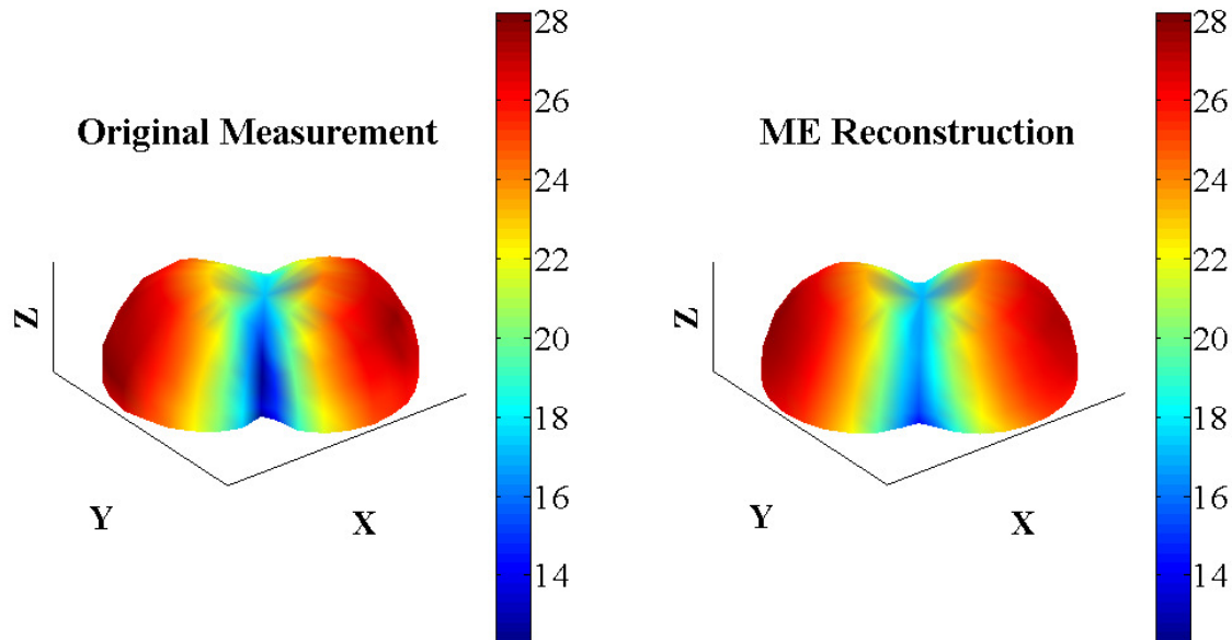
Figure 6-4: A far-field plot of the original pressure measurement and the reconstruction from a ME for a dipole source situated 45^\circ from the x - and y - axes at 550 Hz. The color scale is the same for both plots. Axes units are in dB ref. 20 \mu\text{Pa} .
