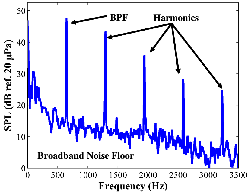
Figure 3-1: The measured power spectrum of a 60-mm fan. The measurement was made 1.5 m from the fan using an on-axis ½" ICP microphone.
